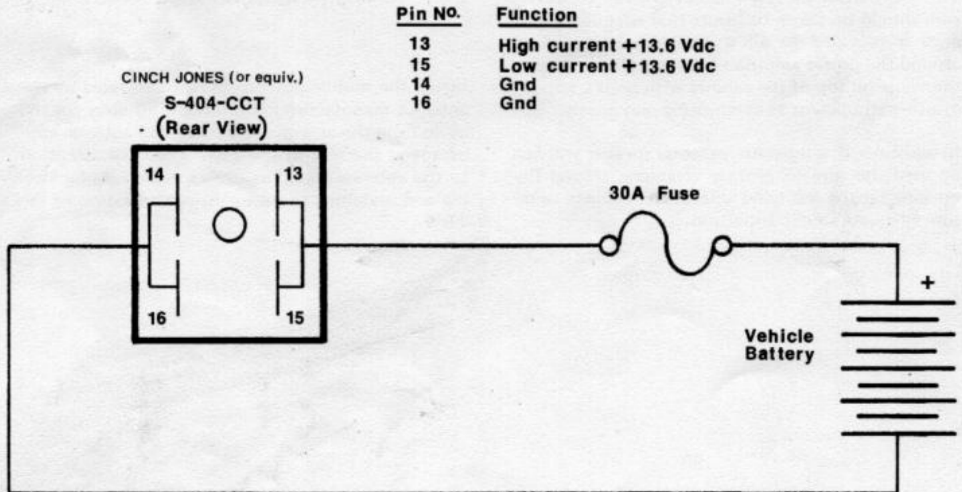
Figure 2-1. TR-7 Power Connection
