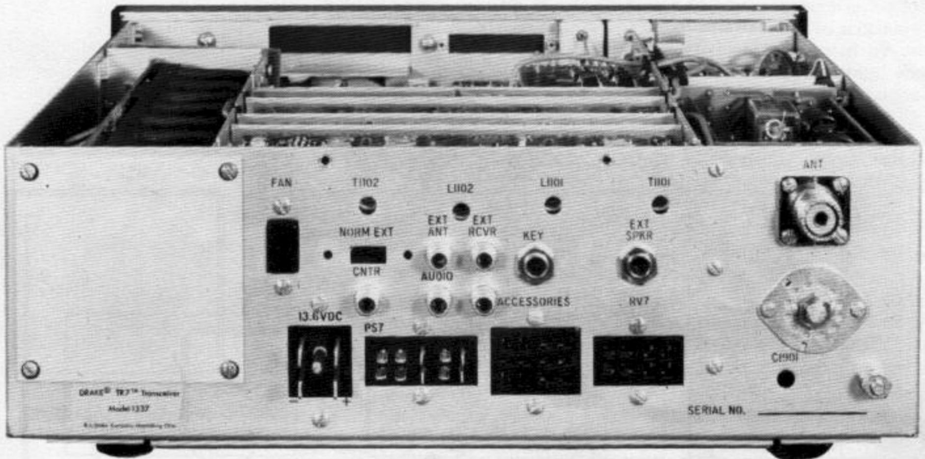
Figure 2-2. TR-7 Rear Panel
