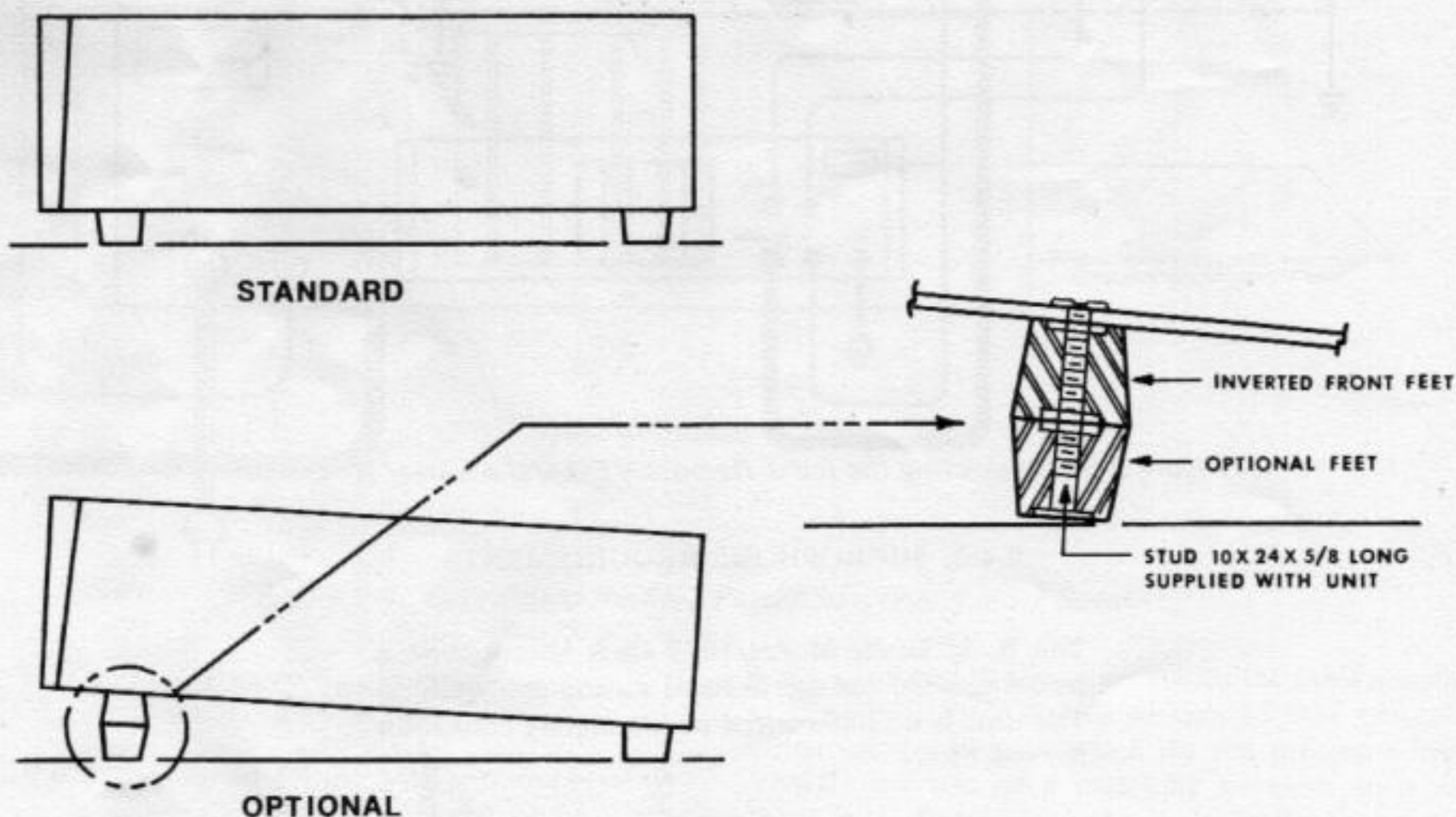
Figure 2-6. Viewing Angle Options
