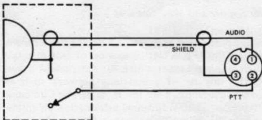
Figure 2-3. TR-7 Microphone Connection
