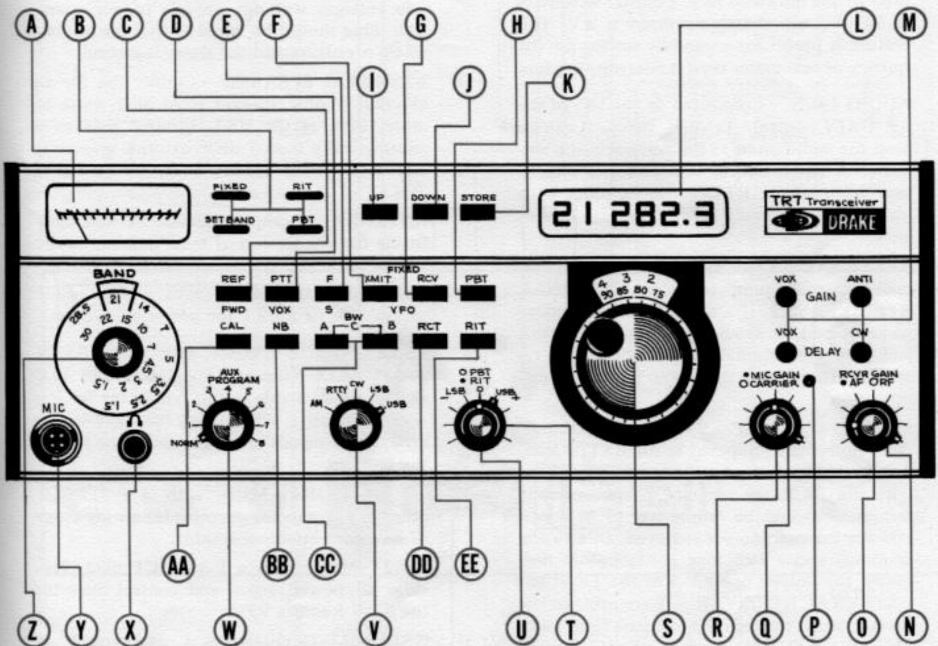
Figure 3-1. Front Panel Controls and Connections
